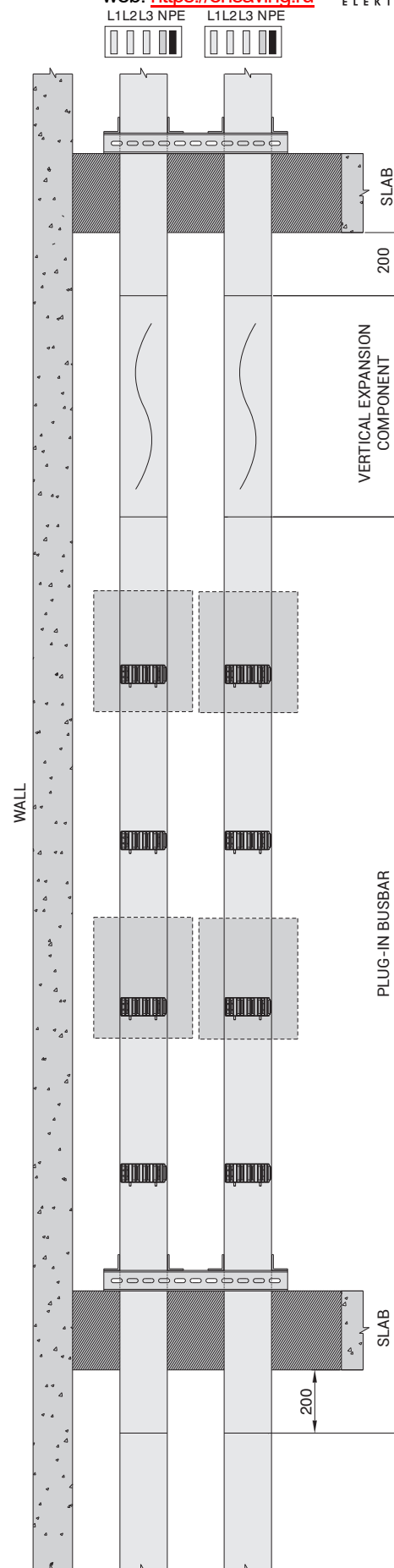
FIGURE-9 MINIMUM DIMENSIONS ON SHAFT APPLICATIONS
