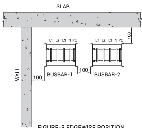
FIGURE-3 EDGEWISE POSITION
