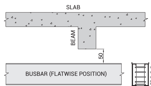
FIGURE-4 SAMPLE WALL CROSSING WITH FIRE BARRIER
