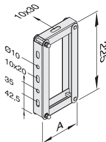
KO-UT Clamp
