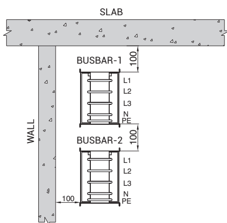
FIGURE-2 FLATWISE POSITION
