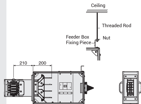
Feeder Box sample equipped with MCCB
